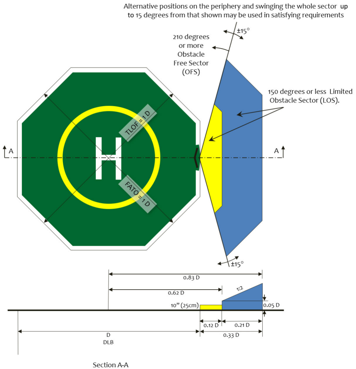
Figure 2: Centralised touchdown markings HSAC Recommended Practice (RP) 2016-1, Revision 2, New Build Helideck Design Guidelines, 2 November 2017
